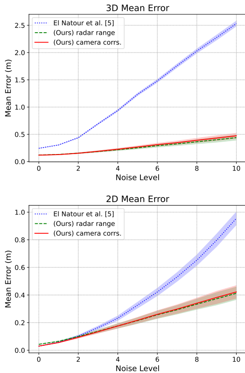
Figure 6: Our methods (overlapping red and green) show resilience to the increasing noise levels for both 2D and 3D reconstruction and achieve a worst case of 0.5 m mean error for 3D reconstruction. Both methods outperform (El Natour et al., 2015a) which performs 5 times worse in 3D reconstruction and 2 times worse in 2D reconstruction at noise level 10.
