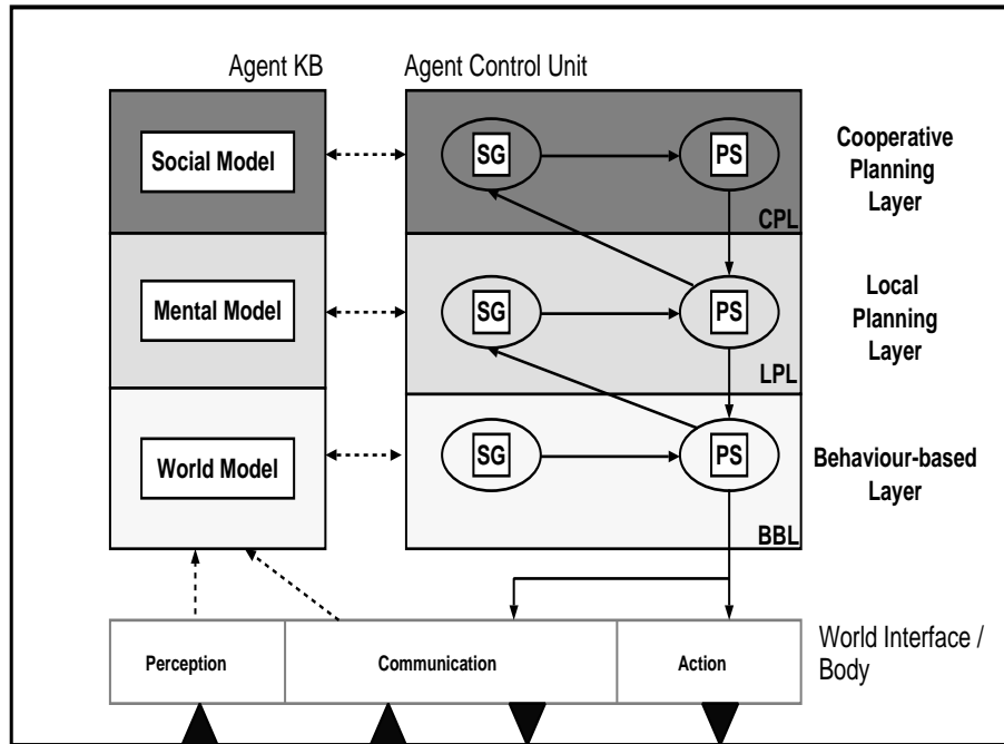
Figure 1: The INTERRAP Agent Architecture
